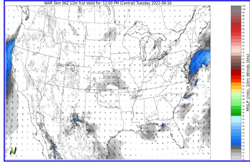
Today's Midday Winds
