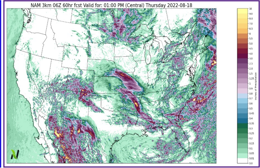
Next 60 Hours of Accumulated Precip
