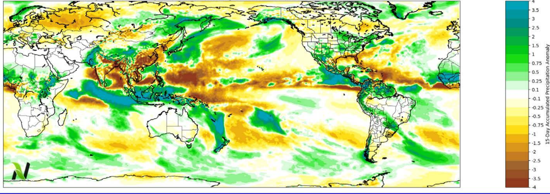
15-day GEFS Precipitation Anomaly from the 00Z GEFS Init.20220816
