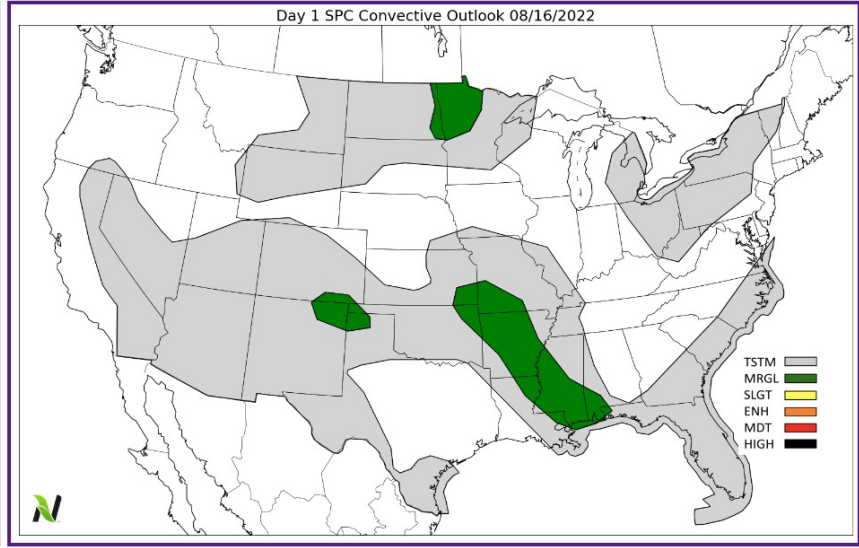
Today's Severe Storm Outlook from the SPC
