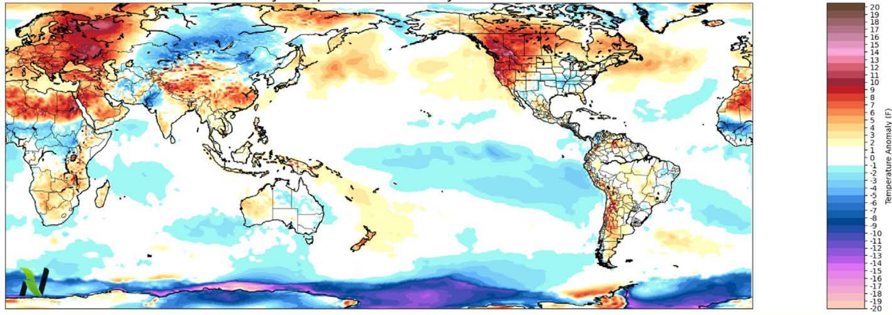
00Z GEFS 15-day Temperature Anomaly Valid Init.20220816
