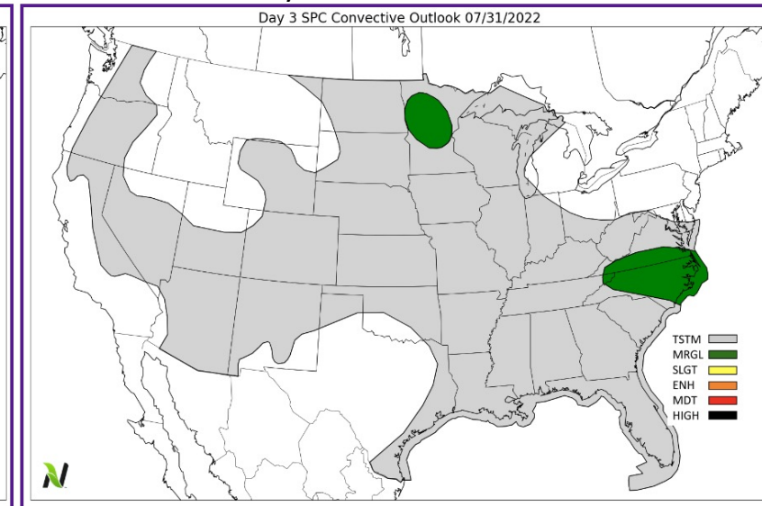
Sunday Severe Storm Outlook
