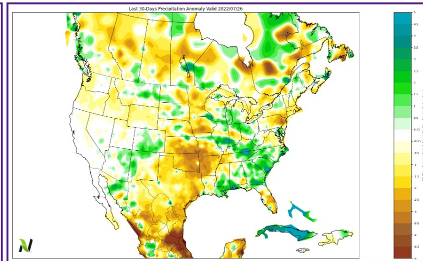
Last 30 Days (North America from CPC)
