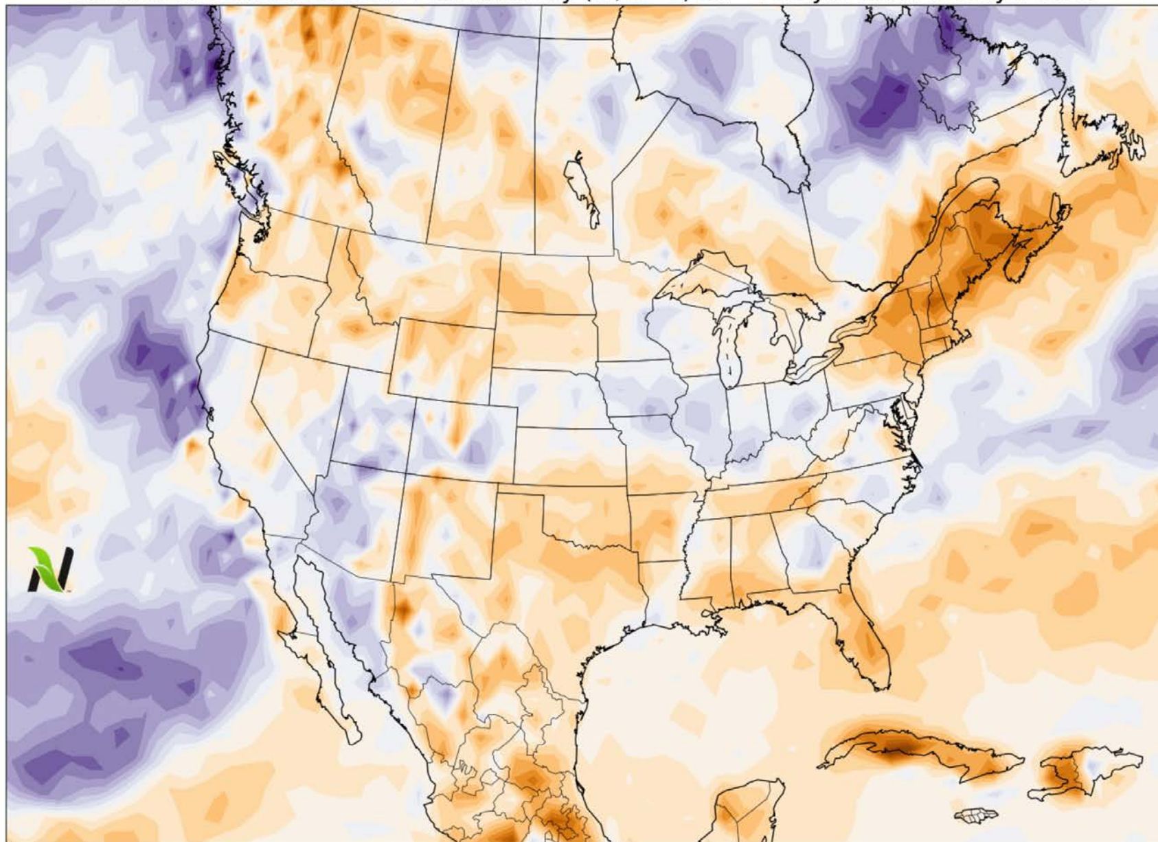
Cumulative Downward Solar Flux Anomaly ( \text{W/m}^2 ) for -->28 Jun 2022 to 28 Jul 2022
