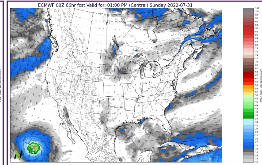
Sunday Severe Storm Outlook
