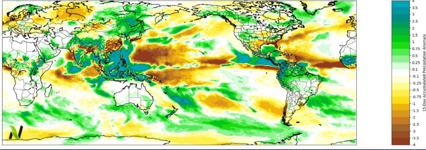
15-day GEFS Precipitation Anomaly from the 00Z GEFS Init.20220729
