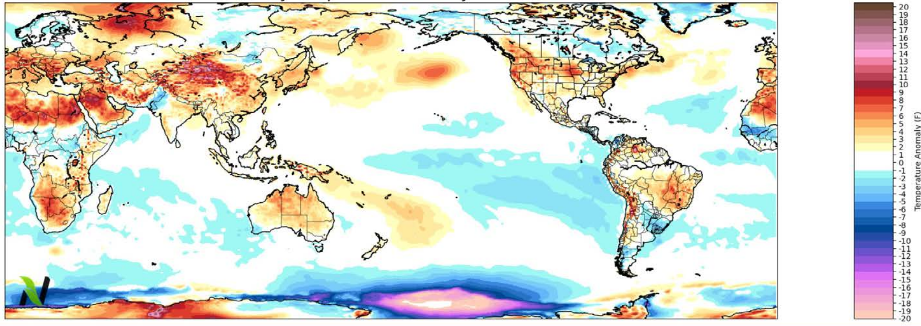
00Z GEFS 15-day Temperature Anomaly Valid Init.20220729
