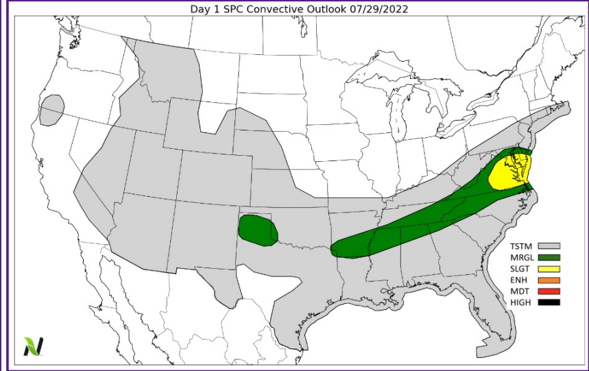
Today's Severe Storm Outlook from the SPC
