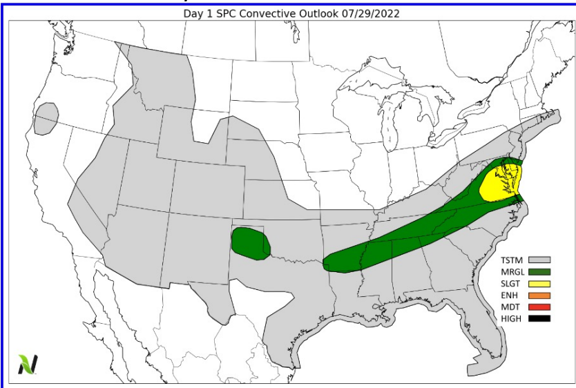
Friday Severe Storms Outlook
