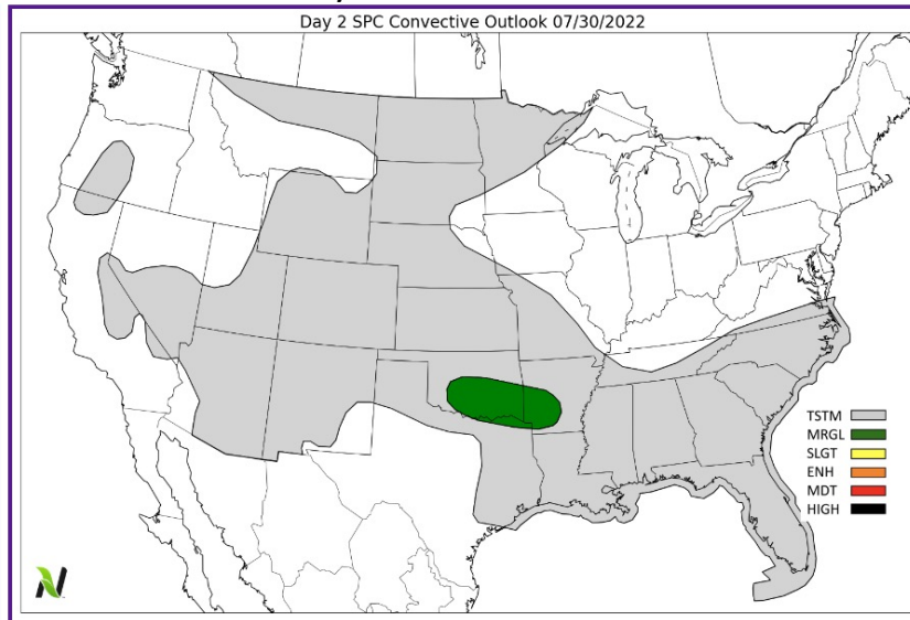
Saturday Severe Storms Outlook
