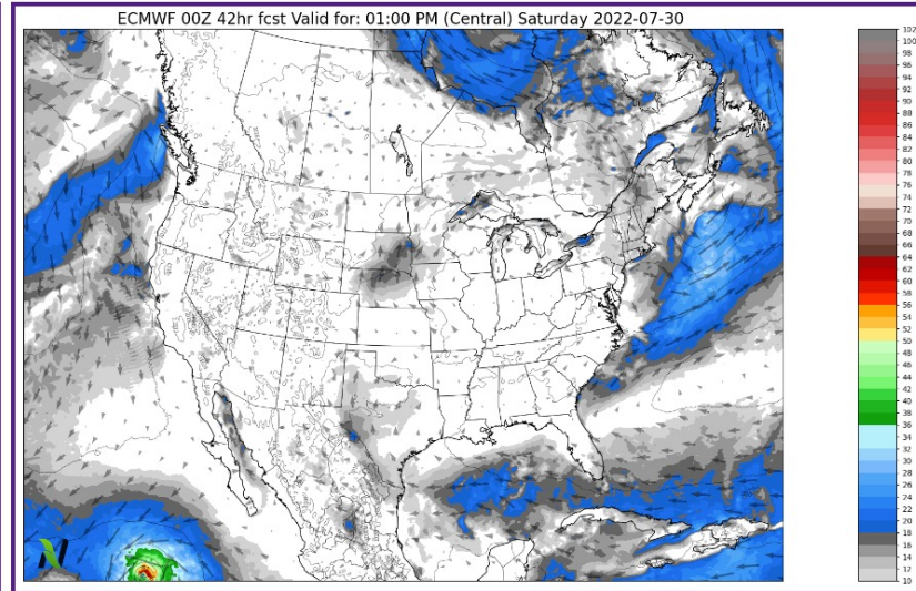
Saturday Severe Storms Outlook
